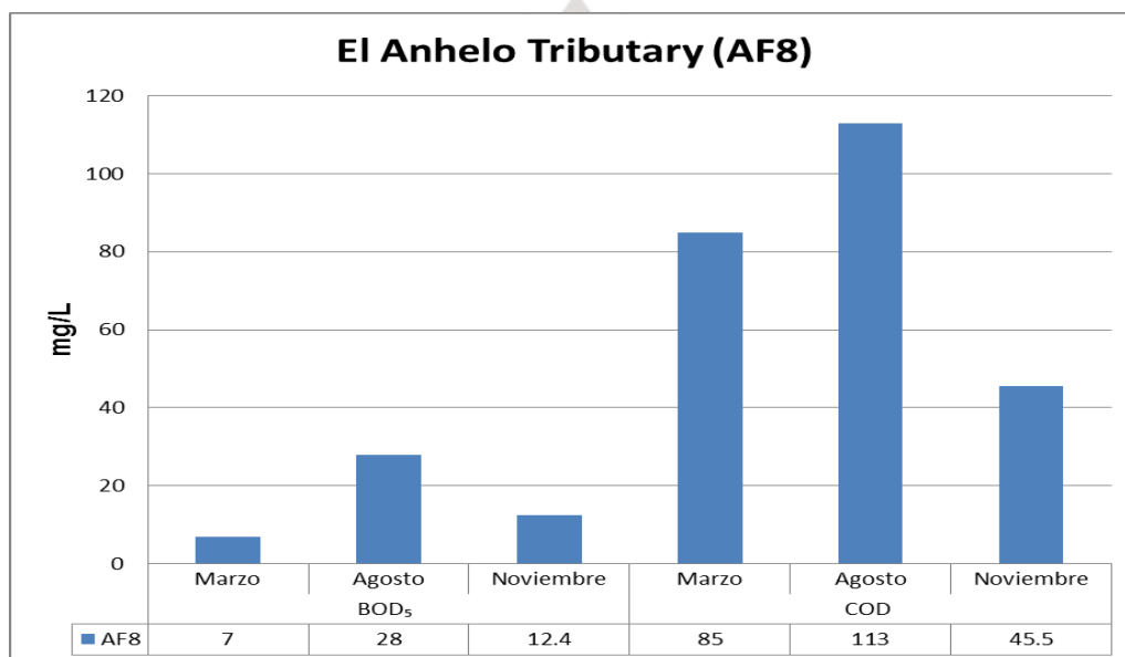
Figure 4: Concentrations of biological oxygen demand and chemical oxygen demand in the tributary
